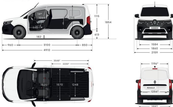
Kangoo Van Dimensions (mm)
