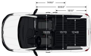
Kangoo Van Dimensions (mm)
