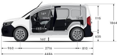
Kangoo Van Dimensions (mm)
