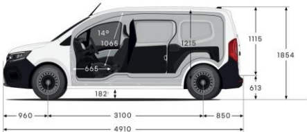
Kangoo Van Dimensions (mm)
