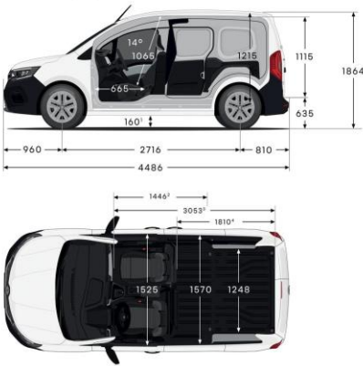
Kangoo Van Dimensions (mm)
