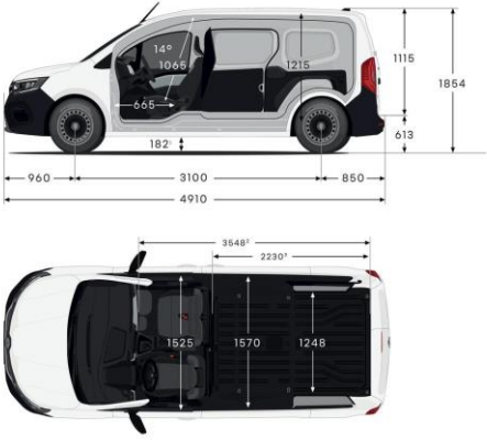
Kangoo Van Dimensions (mm)
